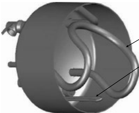
Cut away of a 6 Gallon Heater with a front Heat Exchanger
